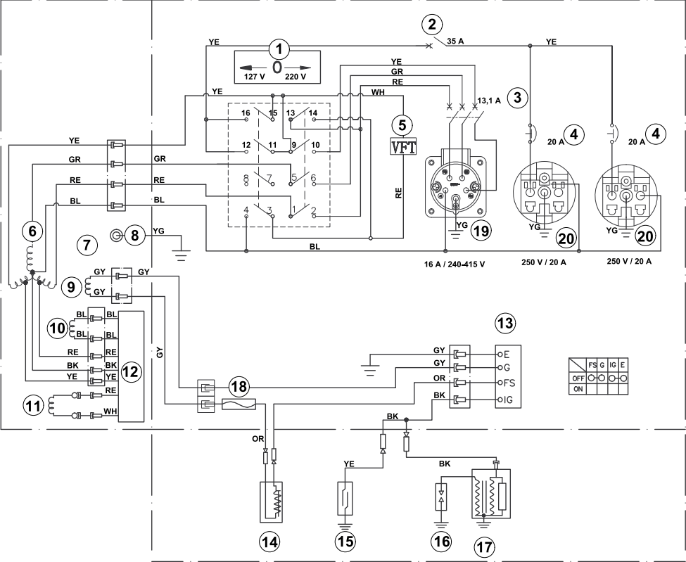
Circuit diagram 127 / 220 V
